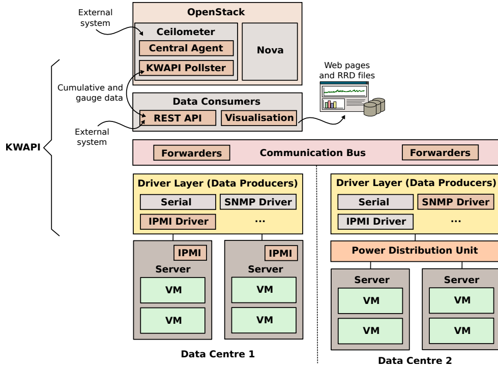
Fig. 2. Overview of KWAPI's architecture.
