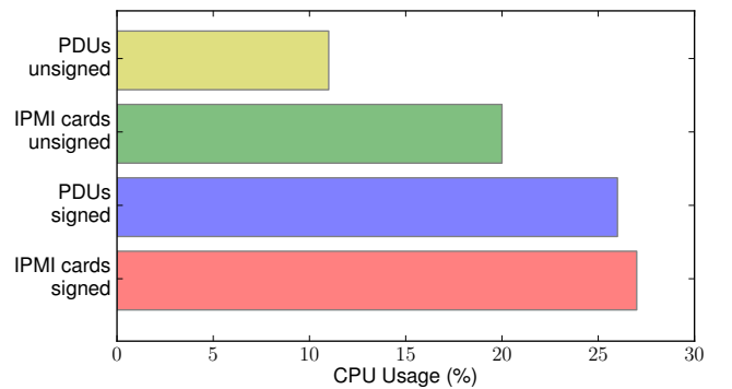
Fig. 5. Driver CPU usage under the evaluated scenarios.
