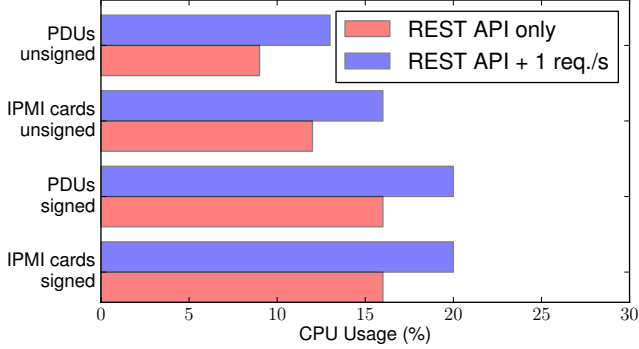
Fig. 6. API consumer CPU usage under the evaluated scenarios.
