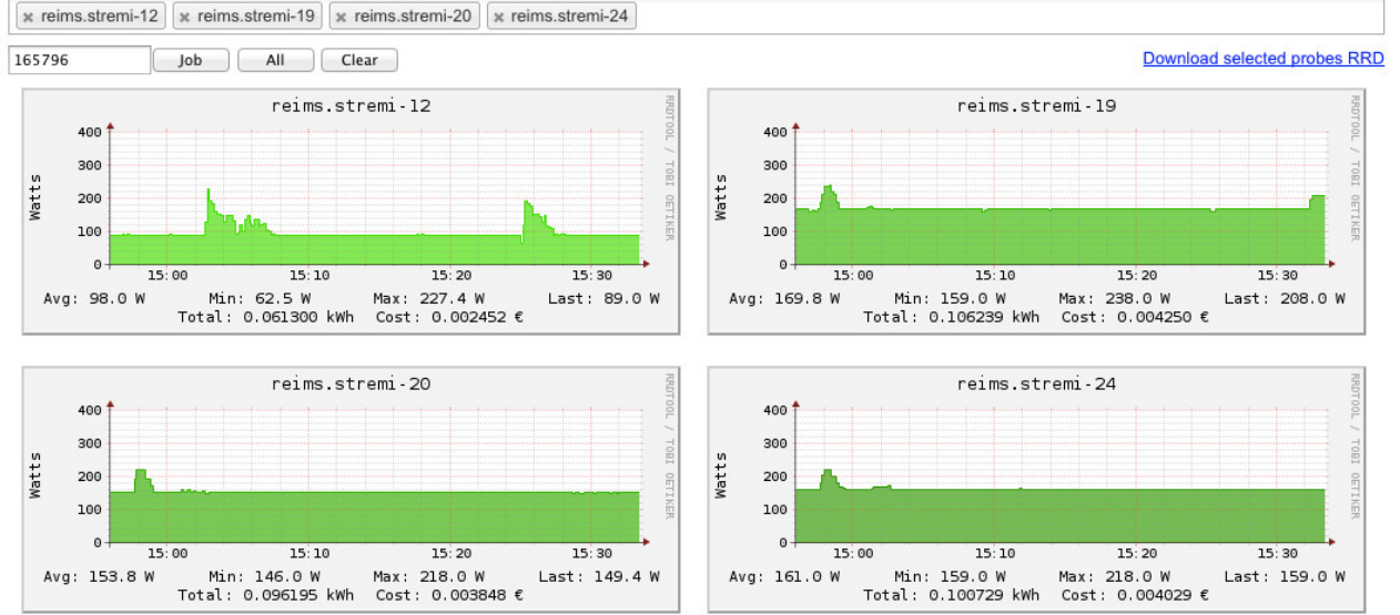
Fig. 4. Example of graph generated by the visualisation plug-in (4 monitored servers).
