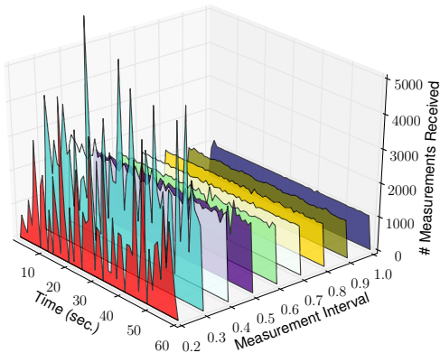
Fig. 7. Number of observations received over a 60 second interval under different multiple intervals.
