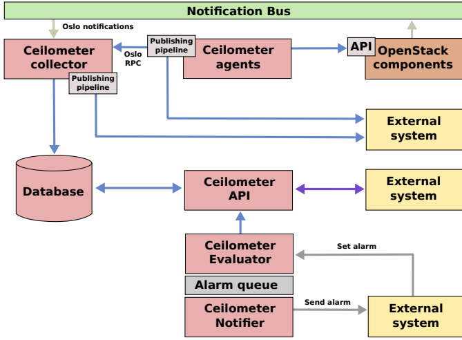
Fig. 1. Overview of Ceilometer's logical architecture.
